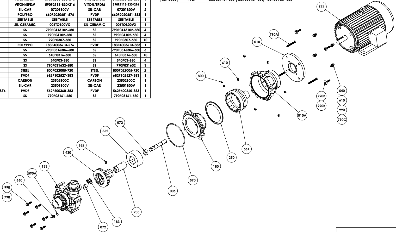
PM-2500 ASSEMBLY_LIT
